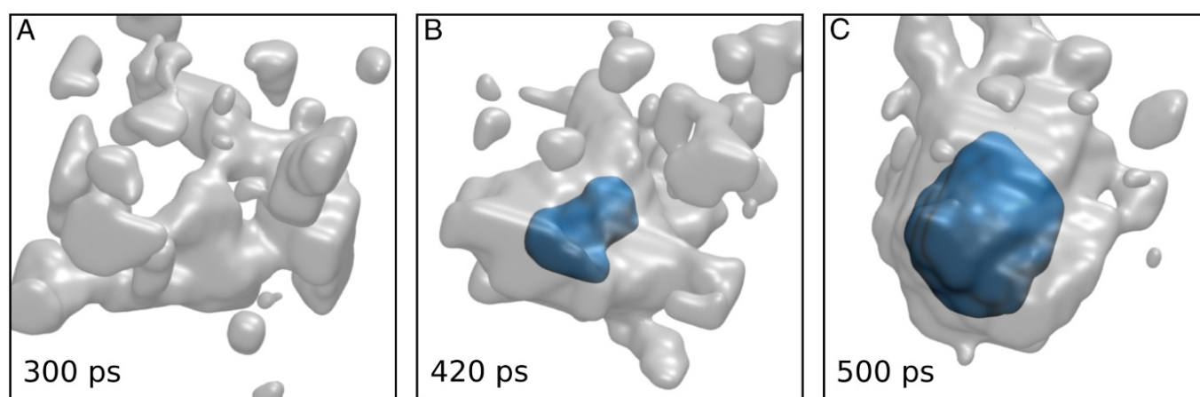
Fig. 3. Ice nucleation occurs in relatively immobile domains of supercooled water. Shown is time evolution of the coarse-grained immobility I(\mathbf{r}) (translucent silver) and crystallinity Q(\mathbf{r}) (opaque blue) fields, from a trajectory harvested by TPS with the mW model. (A) Before nucleation we see large immobile domains and an absence of crystalline order. (B and C) During nucleation, the ice nucleus forms (B) and grows (C) within the immobile domain. The ice cluster in snapshots B and C comprises 83 and 296 molecules, respectively. The diameter of the ice-like region in C is \sim 3.4 nm.
