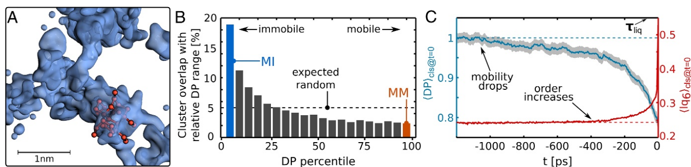
Fig. 2. Connection between DH and precritical cluster formation in the TIP4P/Ice model. (A) Representative snapshot of a spontaneously formed cluster (red bonds and spheres) immersed in the MI region (transparent blue surface representation). (B) Average overlap between the molecules in the largest ice-like cluster and molecules in the relative DP range. Each bar corresponds to a 5% fraction of (sorted) DP values; i.e., the first (last) bar corresponds to the MI (MM) region. The expected overlap if clusters were uncorrelated with the DP would be 5% (indicated by the dashed line). (C) Average evolution of the mobility (DP) and crystallinity ( Iq_6 ) for molecules in a cluster before its first time of assembly (taken to be t = 0 ). Dashed lines indicate the mean values of DP and Iq_6 of the liquid. \tau_{liq} is the structural relaxation time. Shaded regions indicate 95% confidence intervals. All data were obtained with the TIP4P/Ice water model at 240 K.
